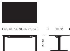
Rectangular Table with T-Foot
